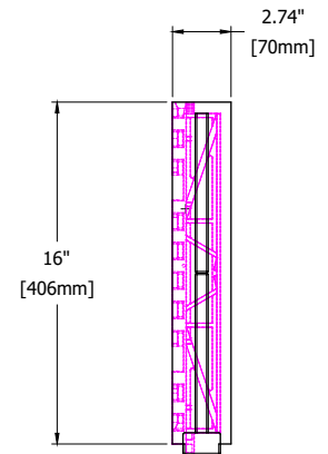
END VIEW
