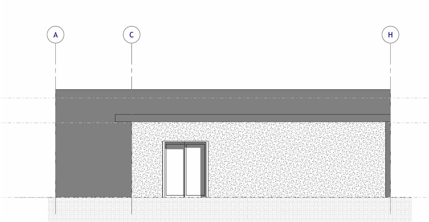
LEFT ELEVATION
