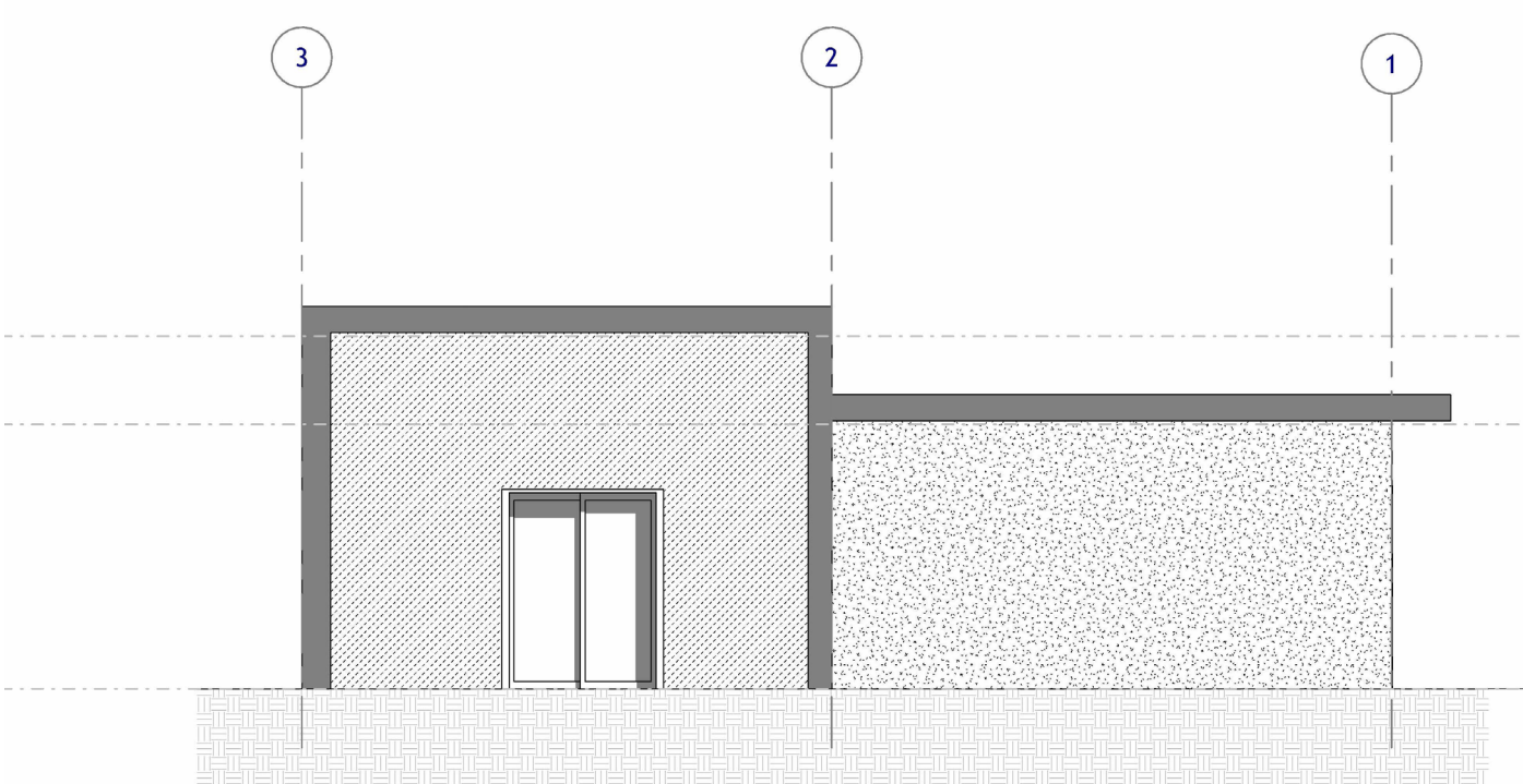
BACK ELEVATION
