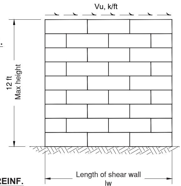
FIGURE 5: ELEVATION
