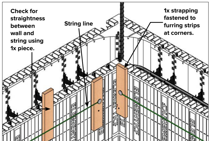
STEP 5: Check building dimensions. Check corners for plumb.
