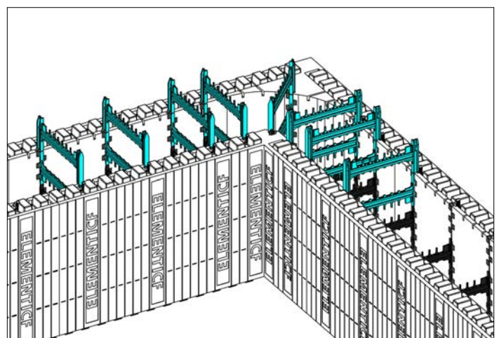
Bridging Flexties at corners. Illustration shows various possible locations, but typically only 2 to 3 bridging Flexties per block are needed.
