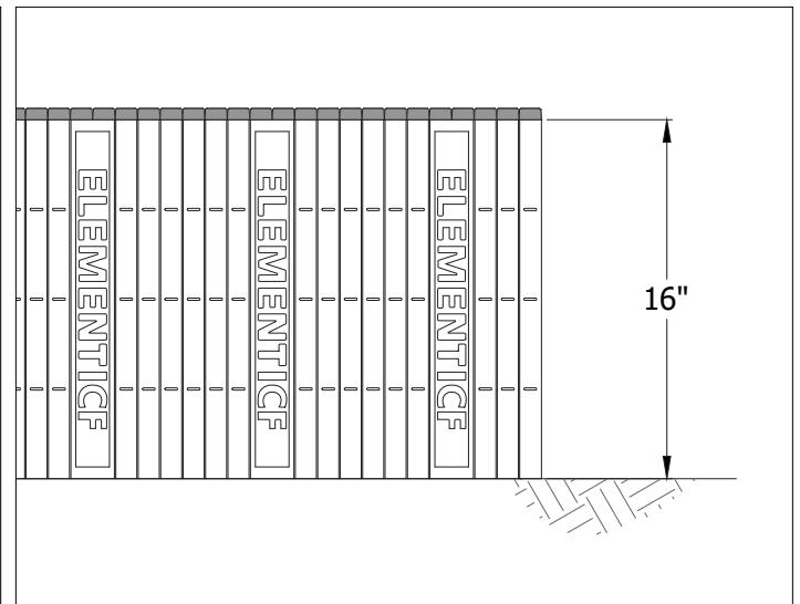
Standard 16 inch tall blocks on footing with bottom interlocks removed.
