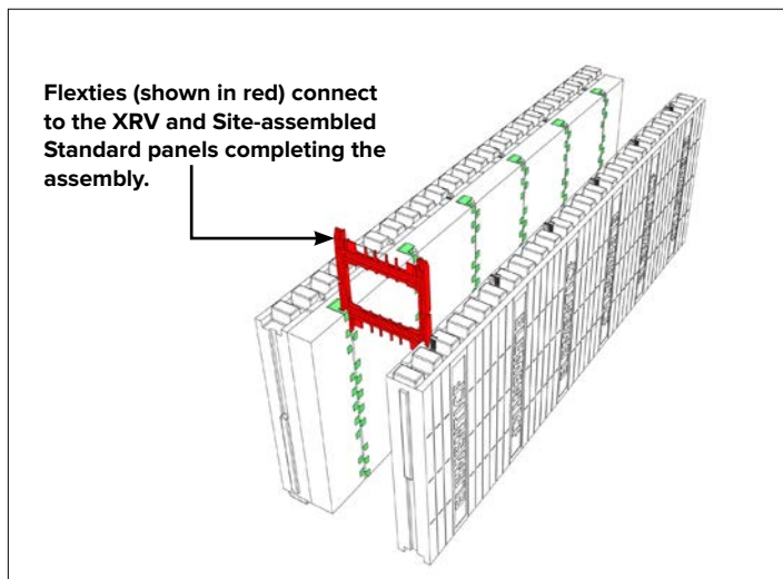
Additional XRV panels can connect to both XRV and Standard panels for progressively increasing R-values.
