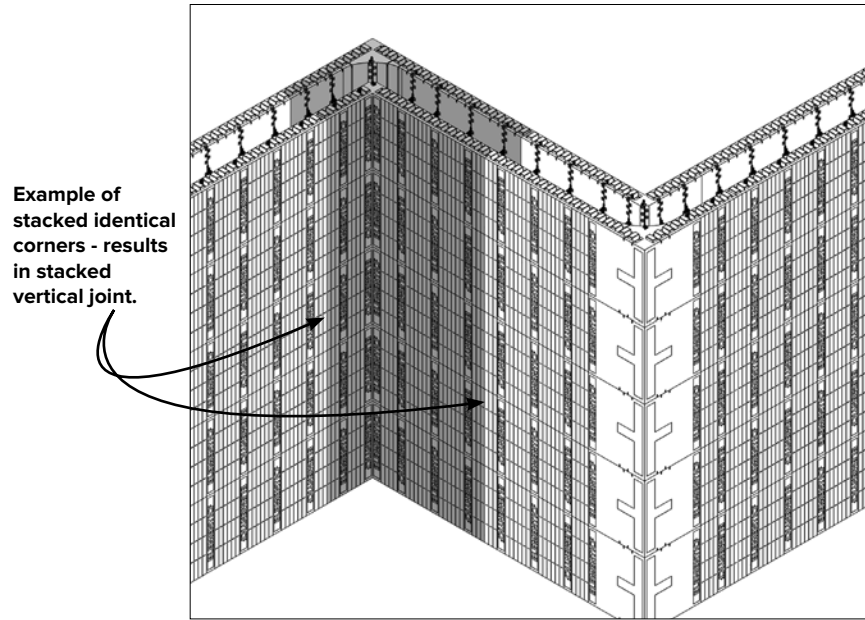
Vertical stacked joints requires additional block support.
