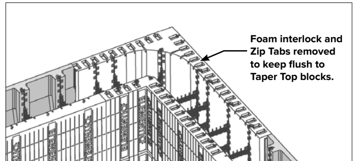
STEP 2: Remove interlock and Zip Tabs.
