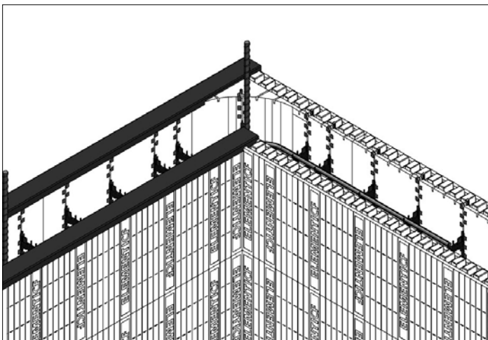
STEP 4: If additional stories are planned, the interlock needs to be protected prior to concrete placement.
