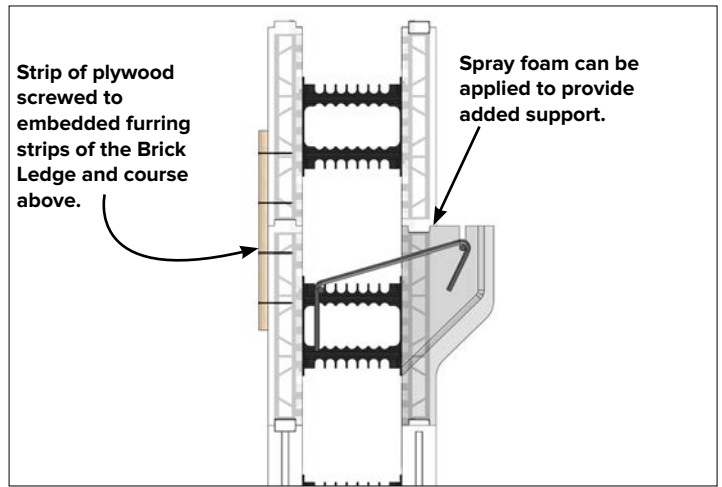
Bottom chord bearing on Element Brick Ledge.
