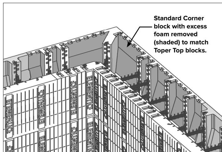
STEP 5: Cut the foam following the cut lines prior to installing in place with a drywall or pruning saw.
