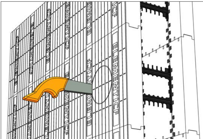
Cut appropriate sized holes for penetrations.
