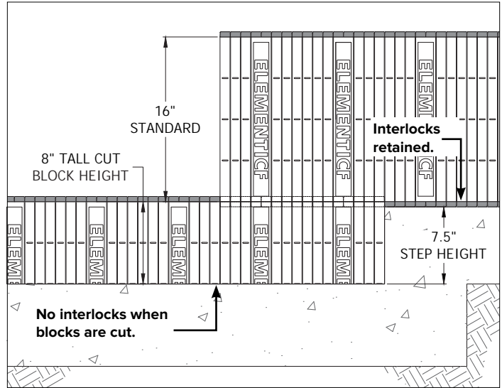
Example of cut block on lower step footing with interlocks retained - reduces step footing by 1/2 inch.
