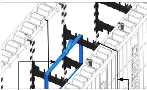
Zip tie securing blocks. Joint between blocks (shown as dark lines for clarity)
