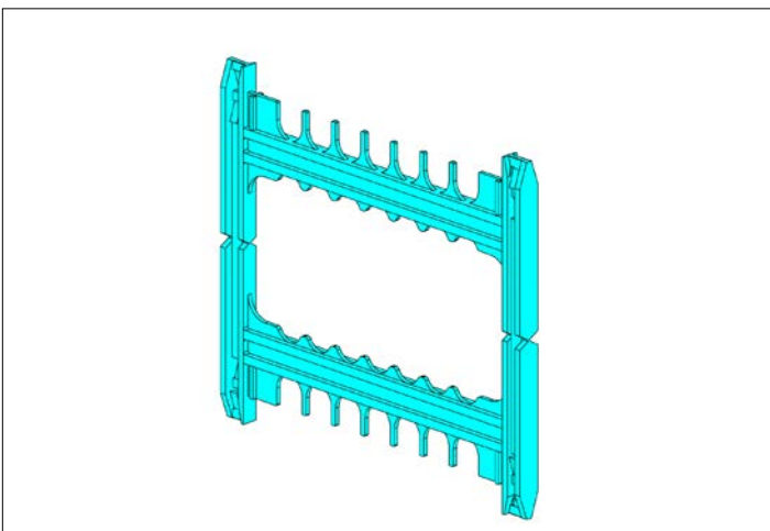
Additional Flexties can be used to increase block pressure resistance (shown in blue for clarity).
