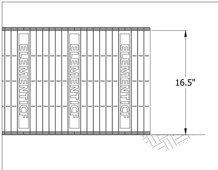
Standard 16 inch tall blocks on footing with bottom interlocks.
