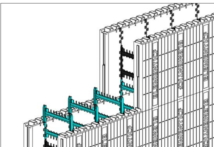
Bridging Flexties added for additional block support. Illustration shows various possible locations, but typically only 2 to 3 bridging Flexties per block are needed.
