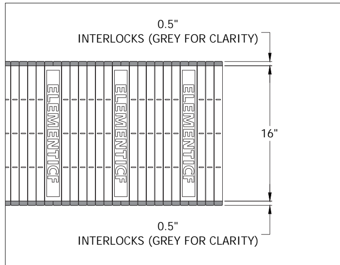
Standard 16 inch tall blocks have interlocks along the top and bottom that are 1/2" in height.
