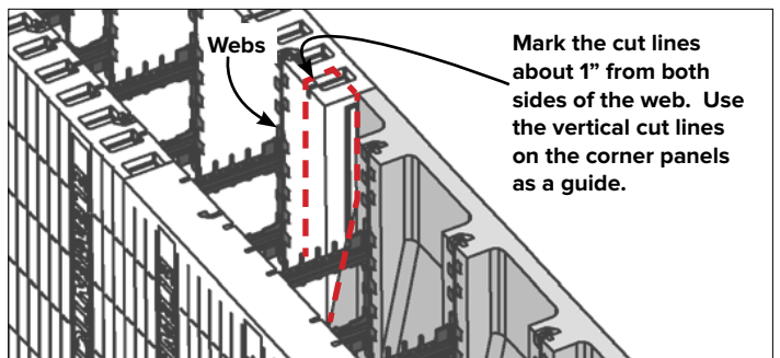
STEP 4: Mark the Standard Corner block to match the Taper Top top profile between all the webs.
