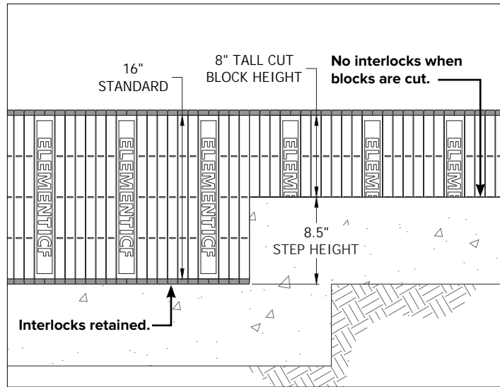
Example of cut block on higher step footing with interlocks in place - increases step footing by 1/2 inch.
