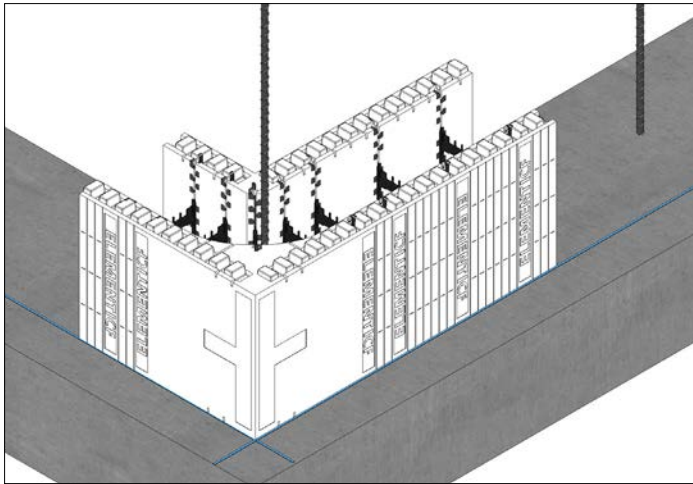
STEP 1: Start first course at a corner and align with chalk line. The interlocks at the bottom of the blocks can be removed, if preferred.
