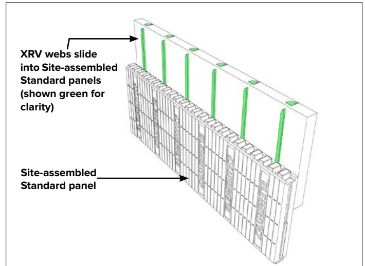
XRV panel connection to Standard Site-assembled panel.
