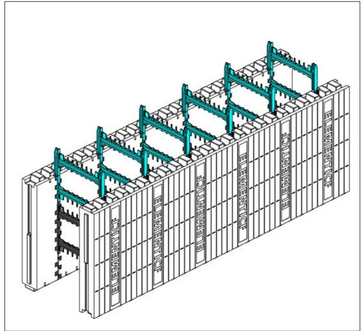
STEP 1: Insert Flexties (shown in blue for clarity).
