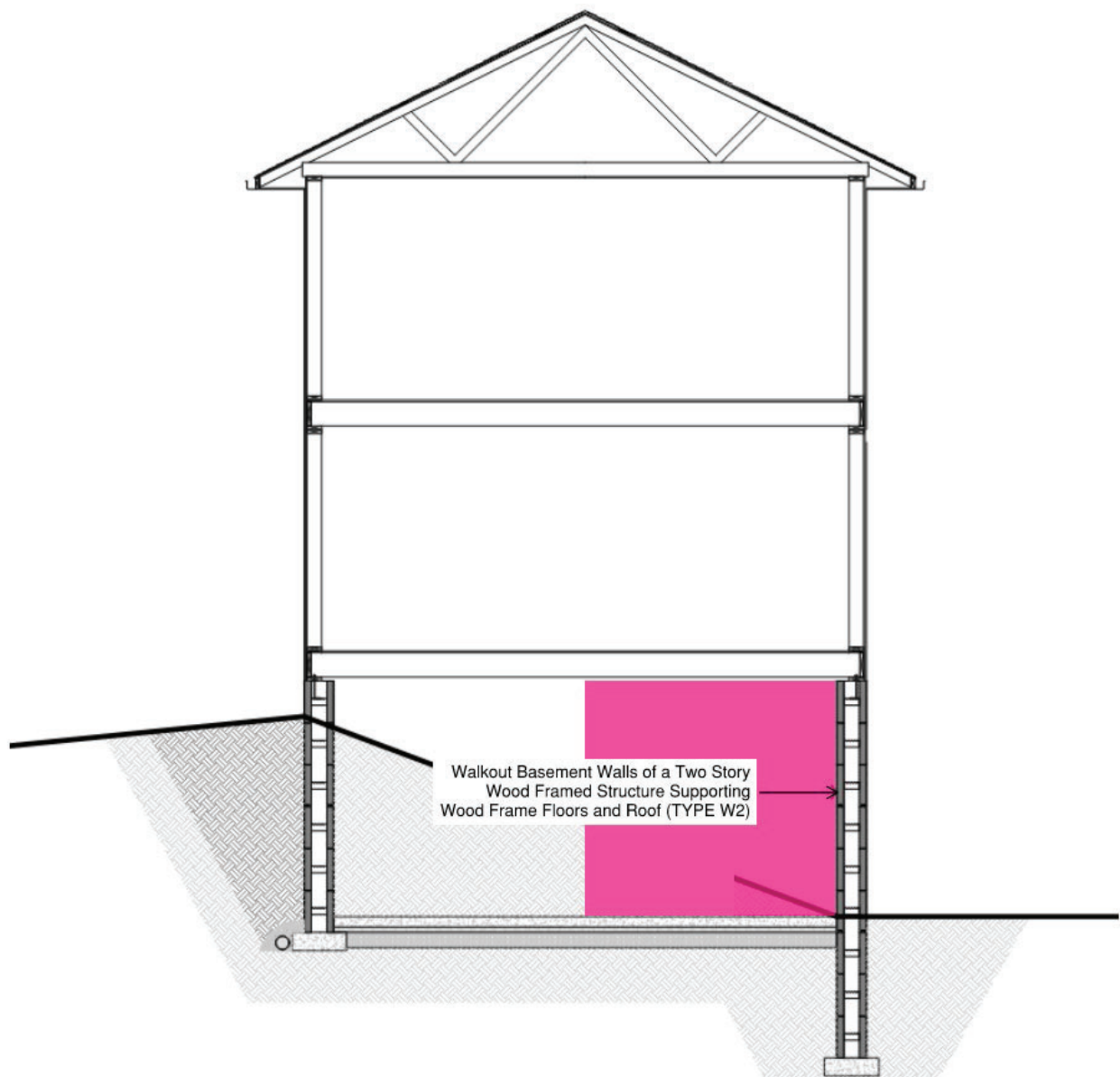
Detail A. 9. 2. Walkout Basement Wall of a Two-Story Wood Framed Structure Supporting Wood Frame Floors and Roof (TYPE W2).
