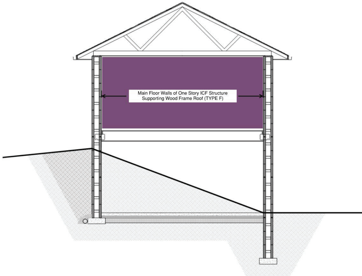
Detail A. 8. 1. Main Floor Walls of One-Story ICF Structure Supporting Wood Frame Roof (TYPE F).
