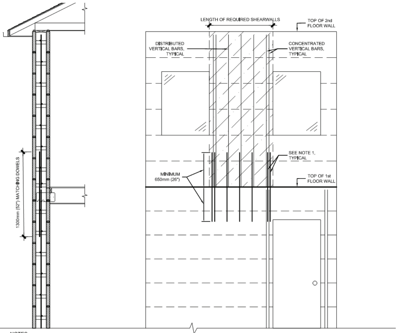
Detail A. 11. Shear Wall Dowels.
