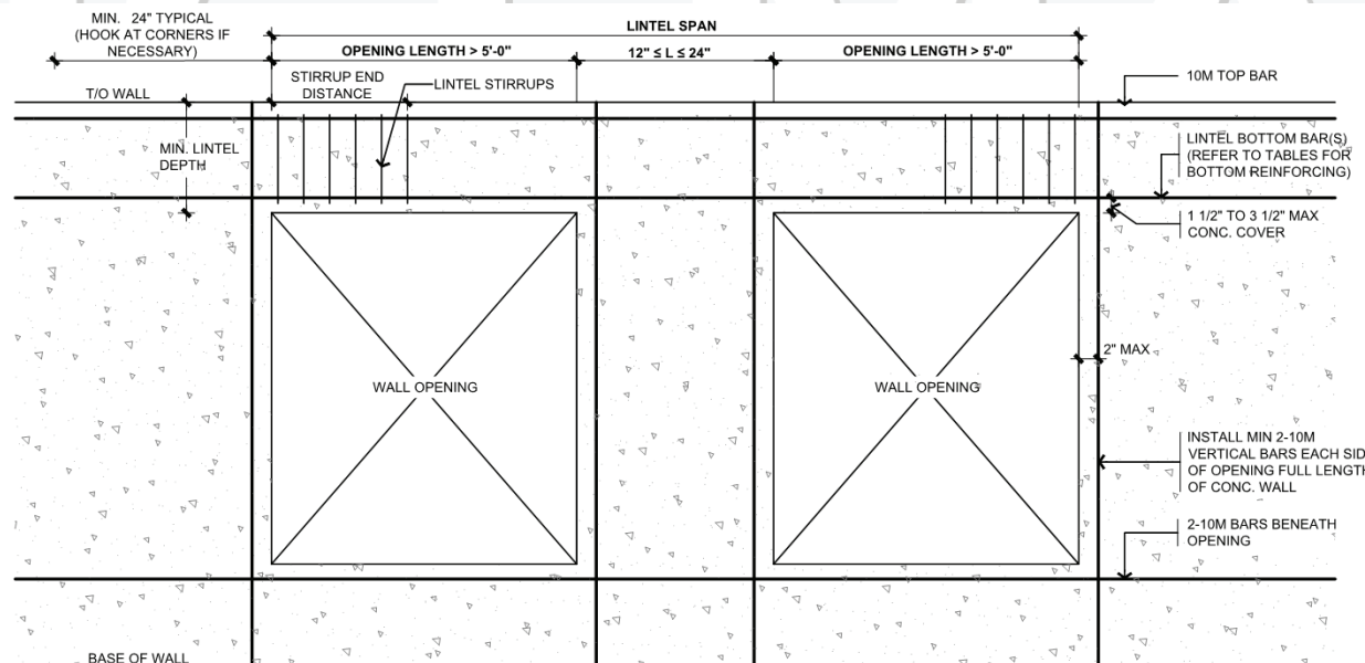
Detail L. 5. Lintel Span with Less Than 610mm (24") of Wall Between Openings, and Openings Are Greater Than 1.53m (5'-0") in Length.
