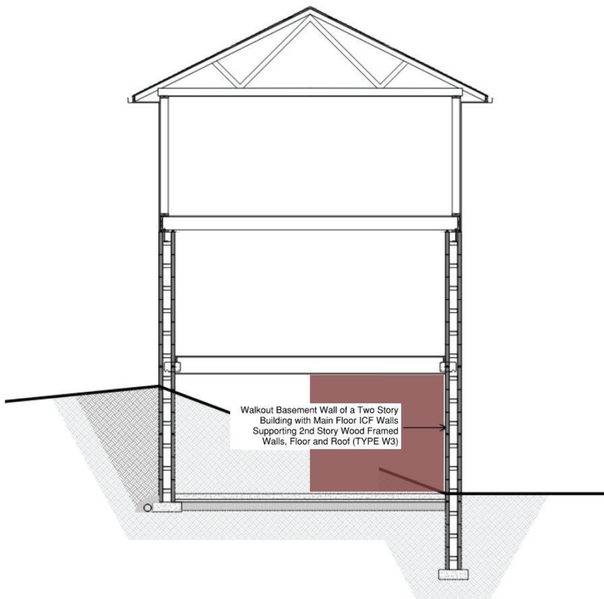
Detail A. 9. 3. Walkout Basement Wall of a Two-Story Building with Main Floor ICF Walls Supporting Second Story Wood Framed Walls, Floor and Roof (TYPE W3).
