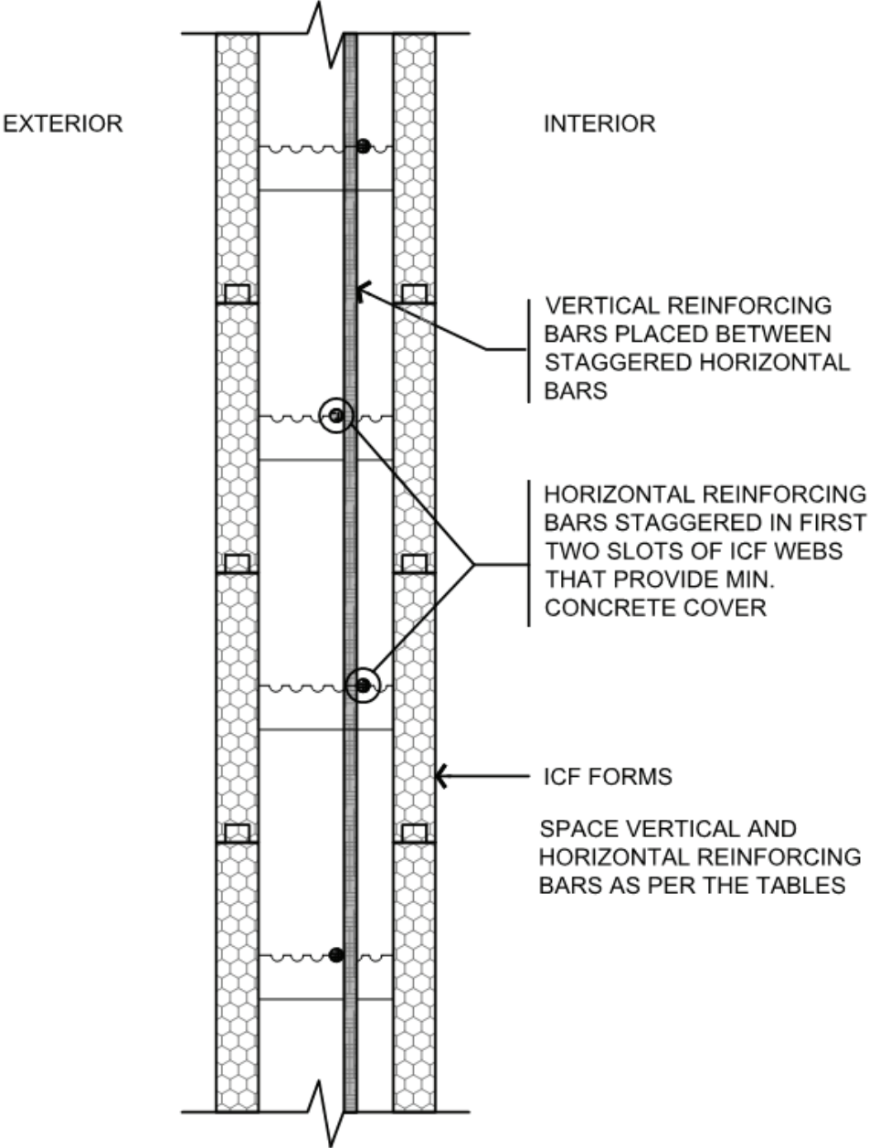
Detail B. 1. Below Grade Wall Reinforcing Placement for All Wall Thicknesses.
