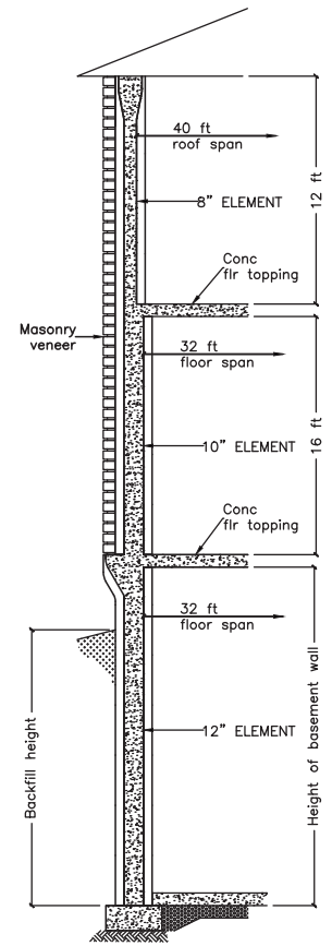
Fig 2D Assumed typical flooring, wall & roof for Table 2D. Height & thickness of above-grade walls, floor & roof spans, including materials (i.e., wood frame, concrete, and cladding) can vary provided the total factored load on basement wall does not exceed 9 kips/ft.
