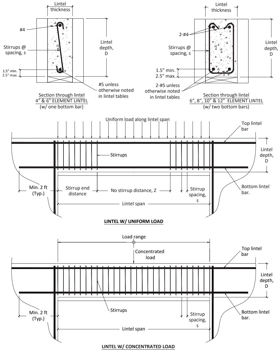
Fig 4 Lintel reinforcement
